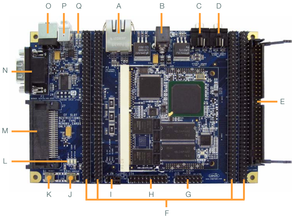
Figure 2.2 – Connection Diagram for the Application Baseboard
